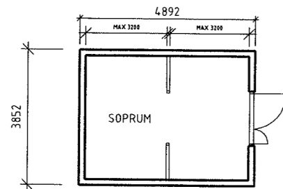
PLAN SOPHUS
